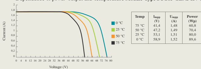
Dependence of power output and temperature Module Type SCG85-GEN2-HV-F
